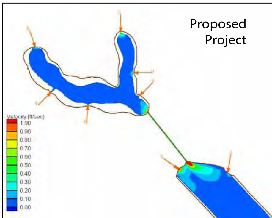
Figure 3.9-1 Maximum Velocity Distribution During 10-Year Flood Event
