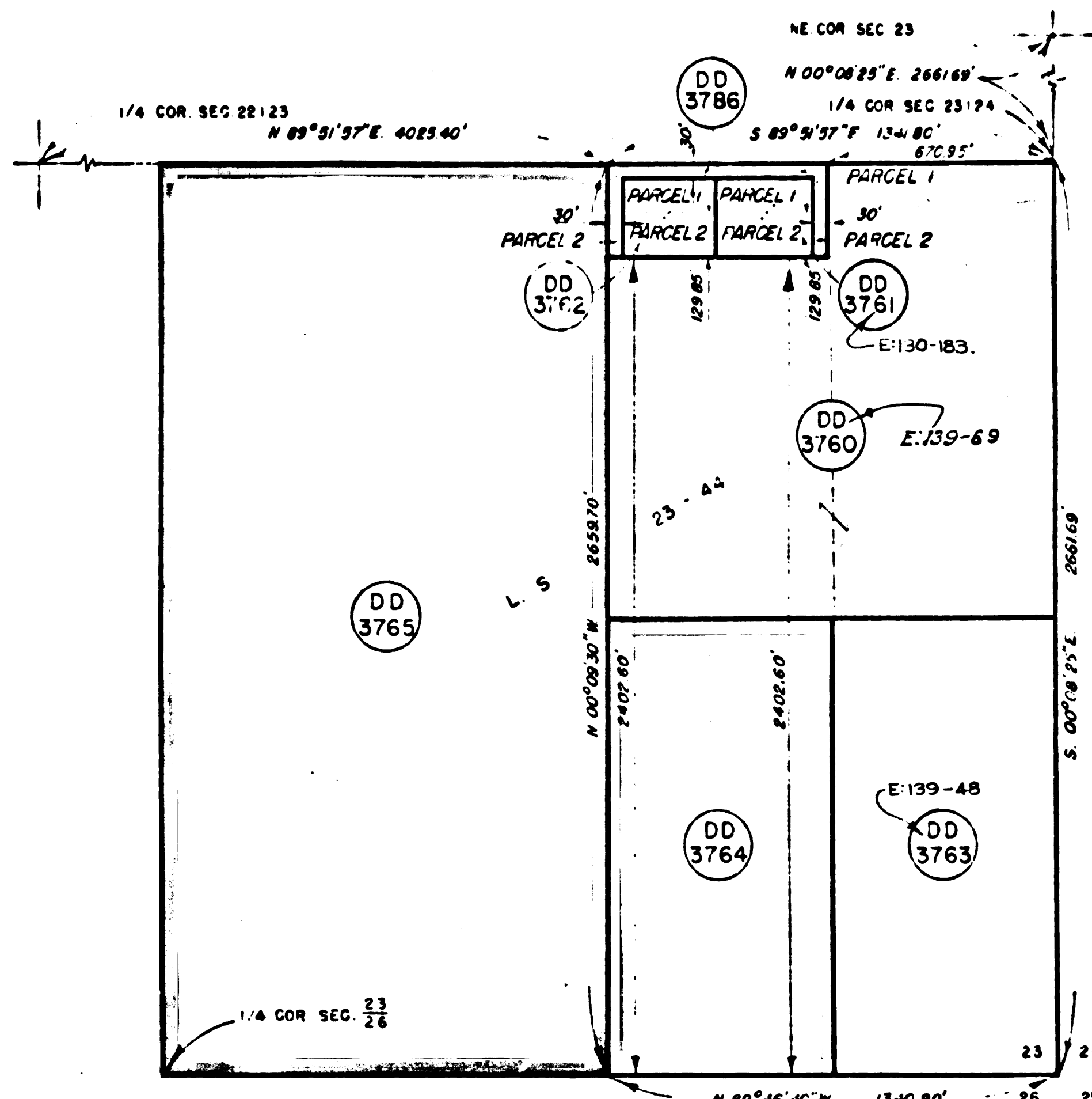
DETAIL "A"
