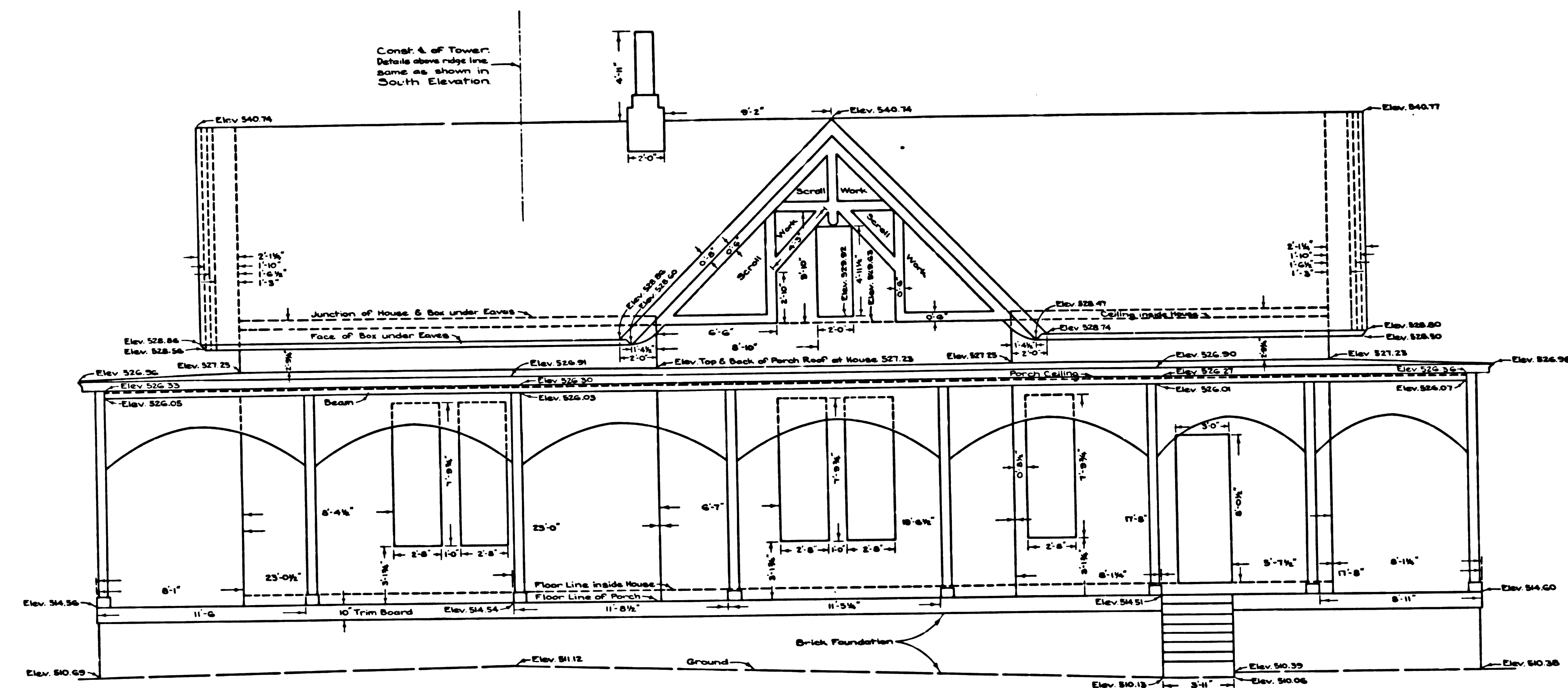
EAST ELEVATION
