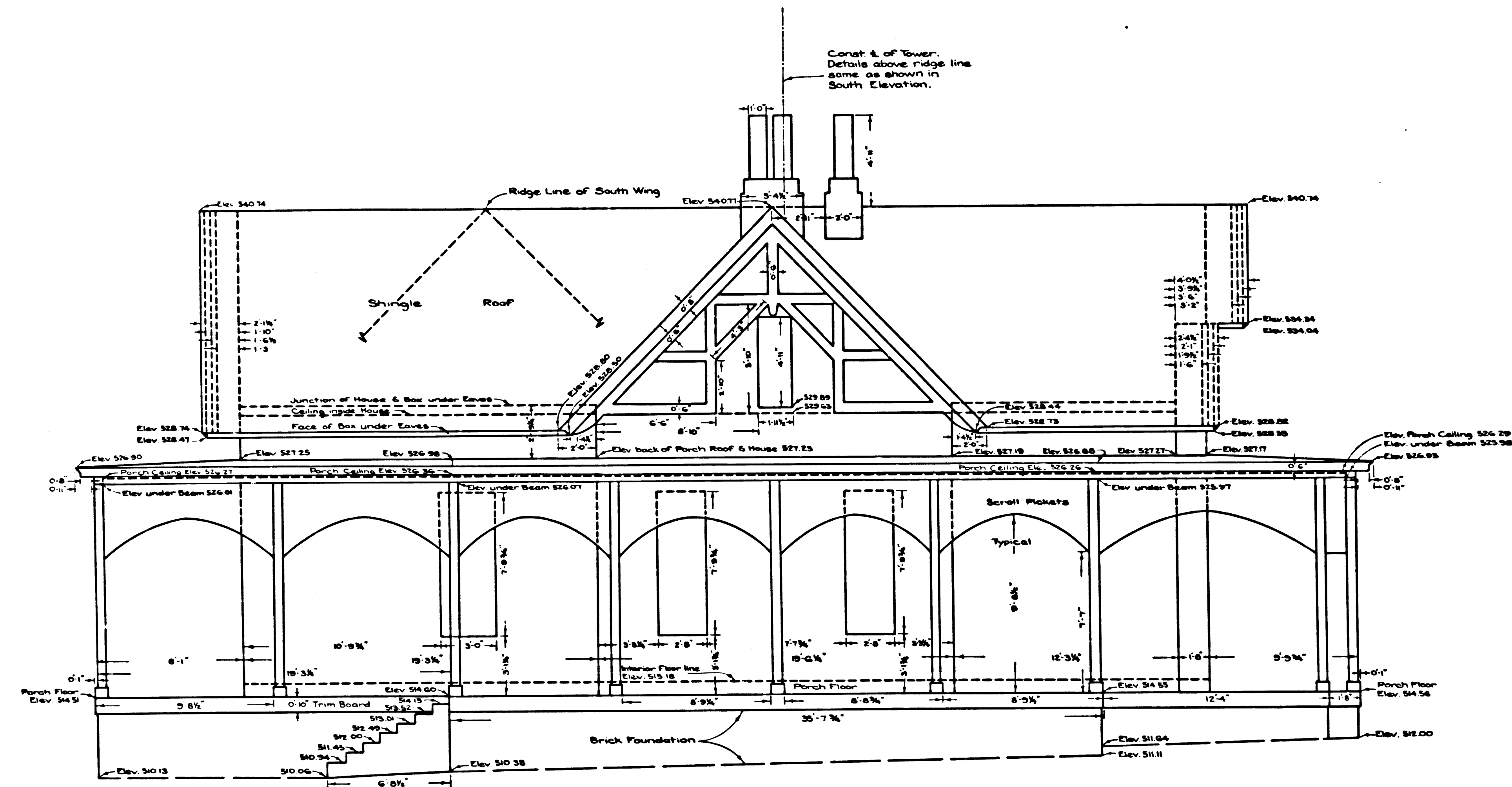
NORTH ELEVATION
