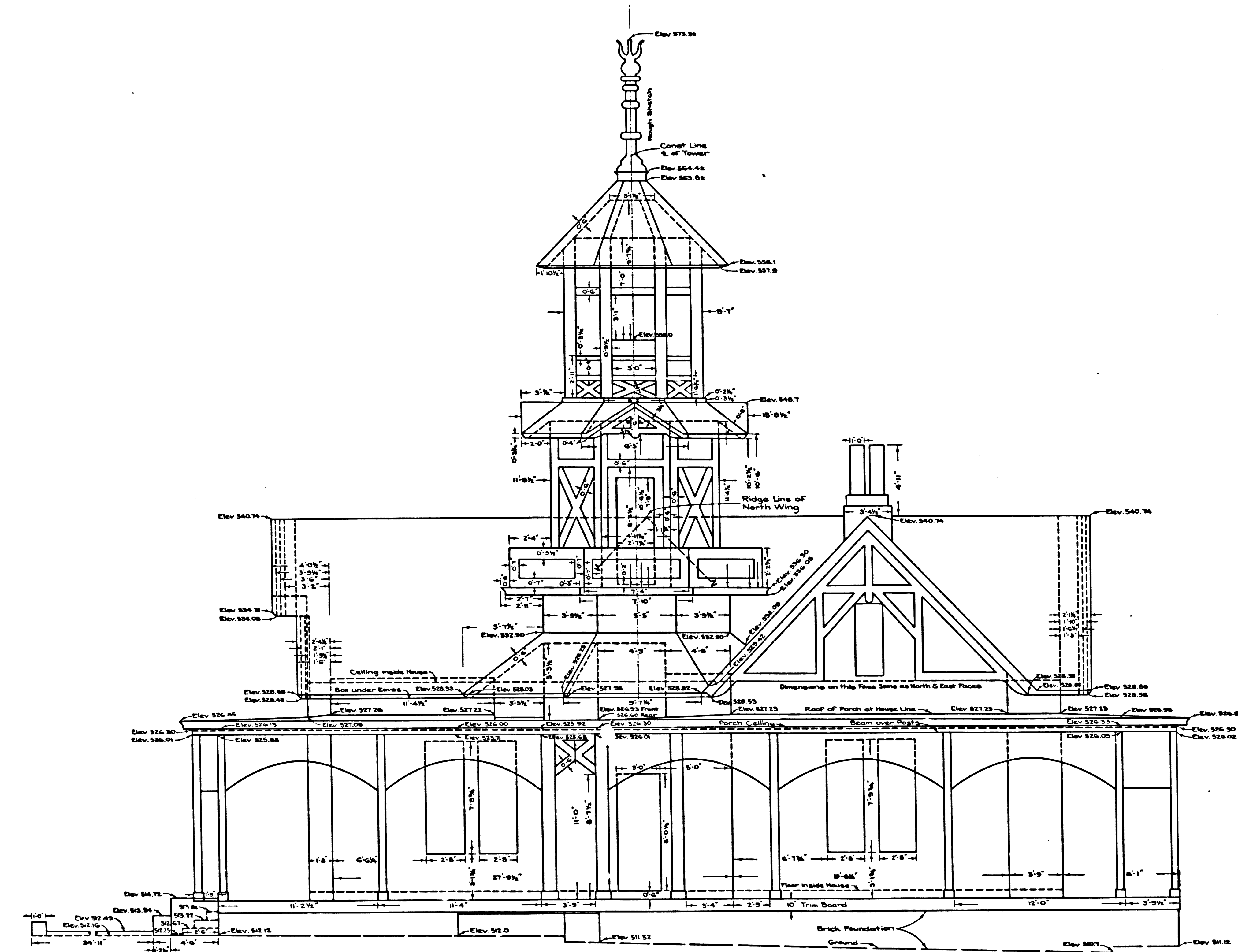
SOUTH ELEVATION
