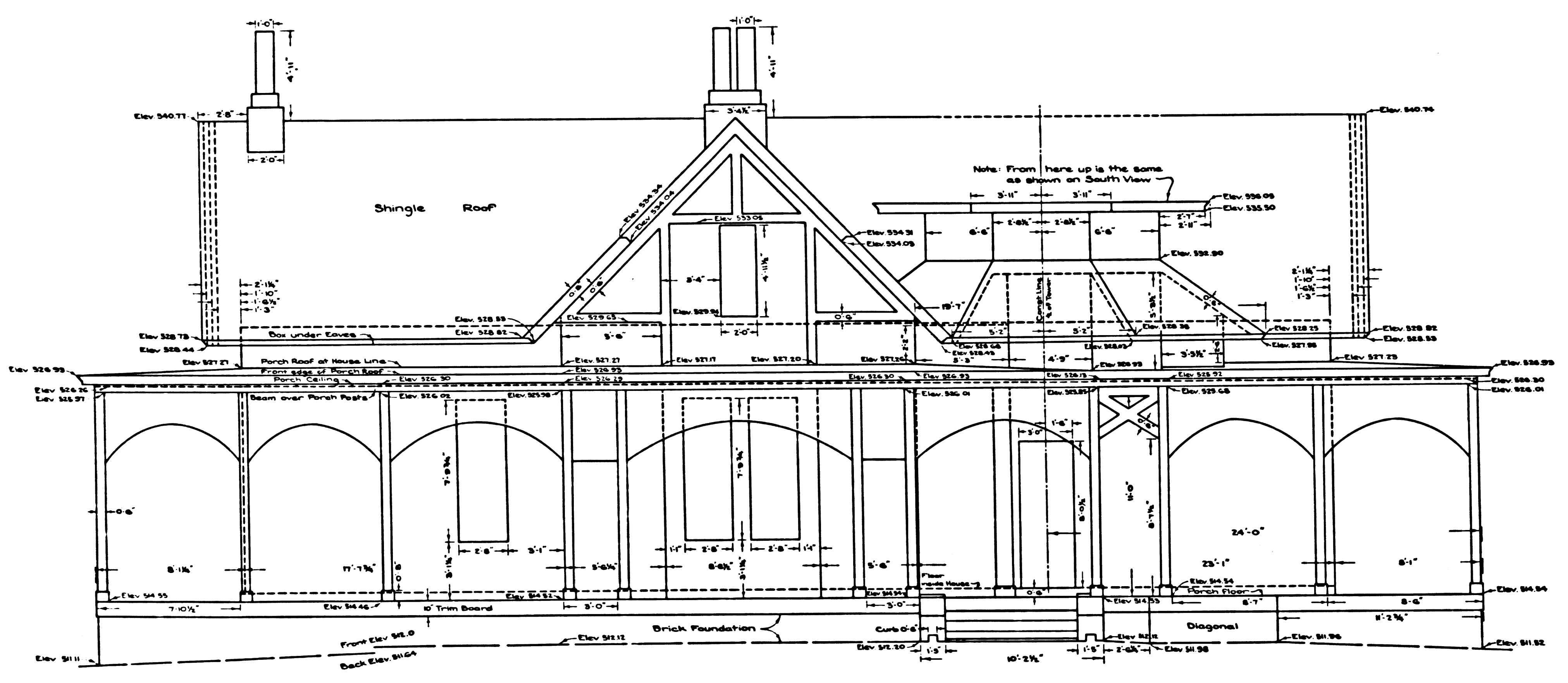
WEST ELEVATION
