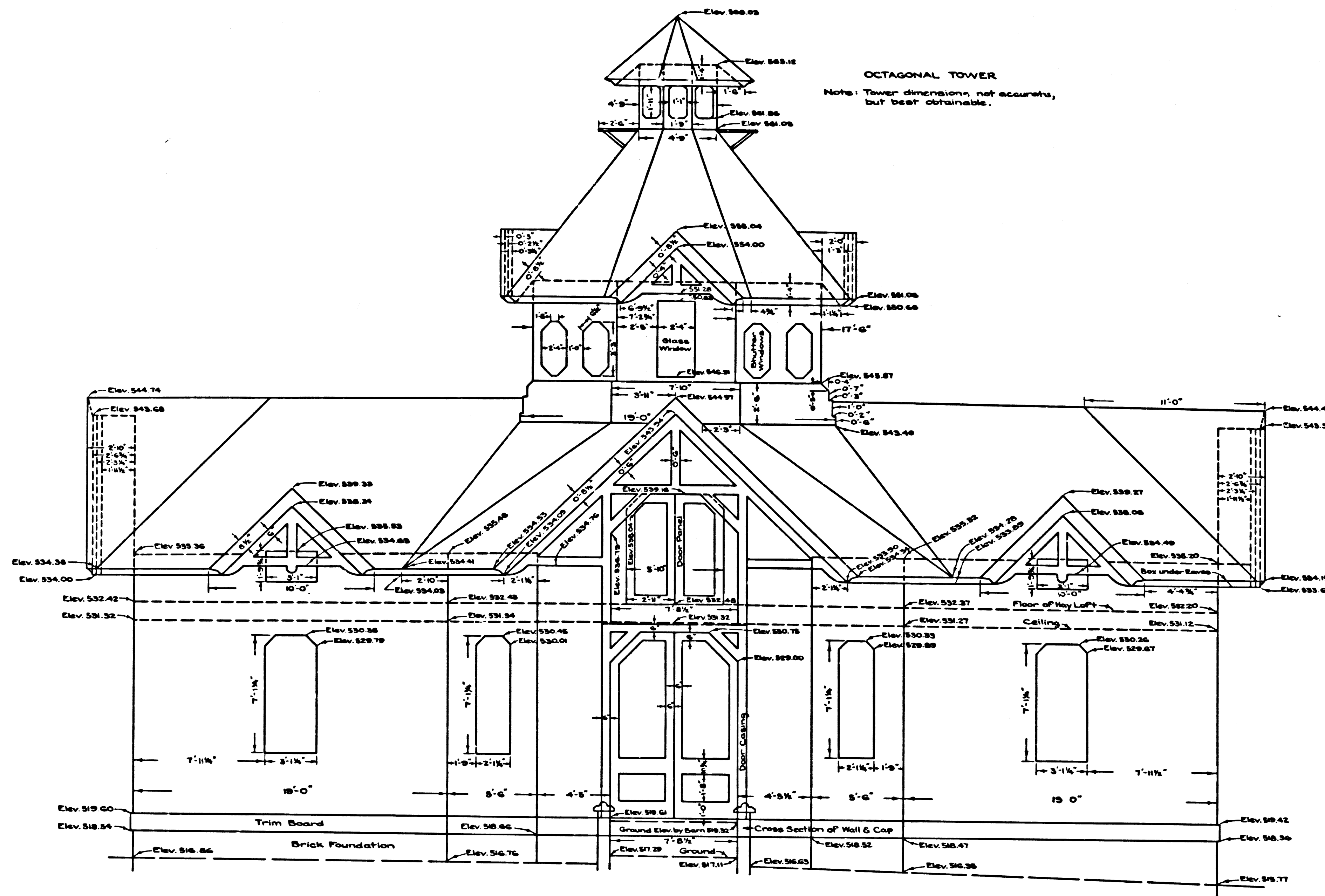
EAST ELEVATION
