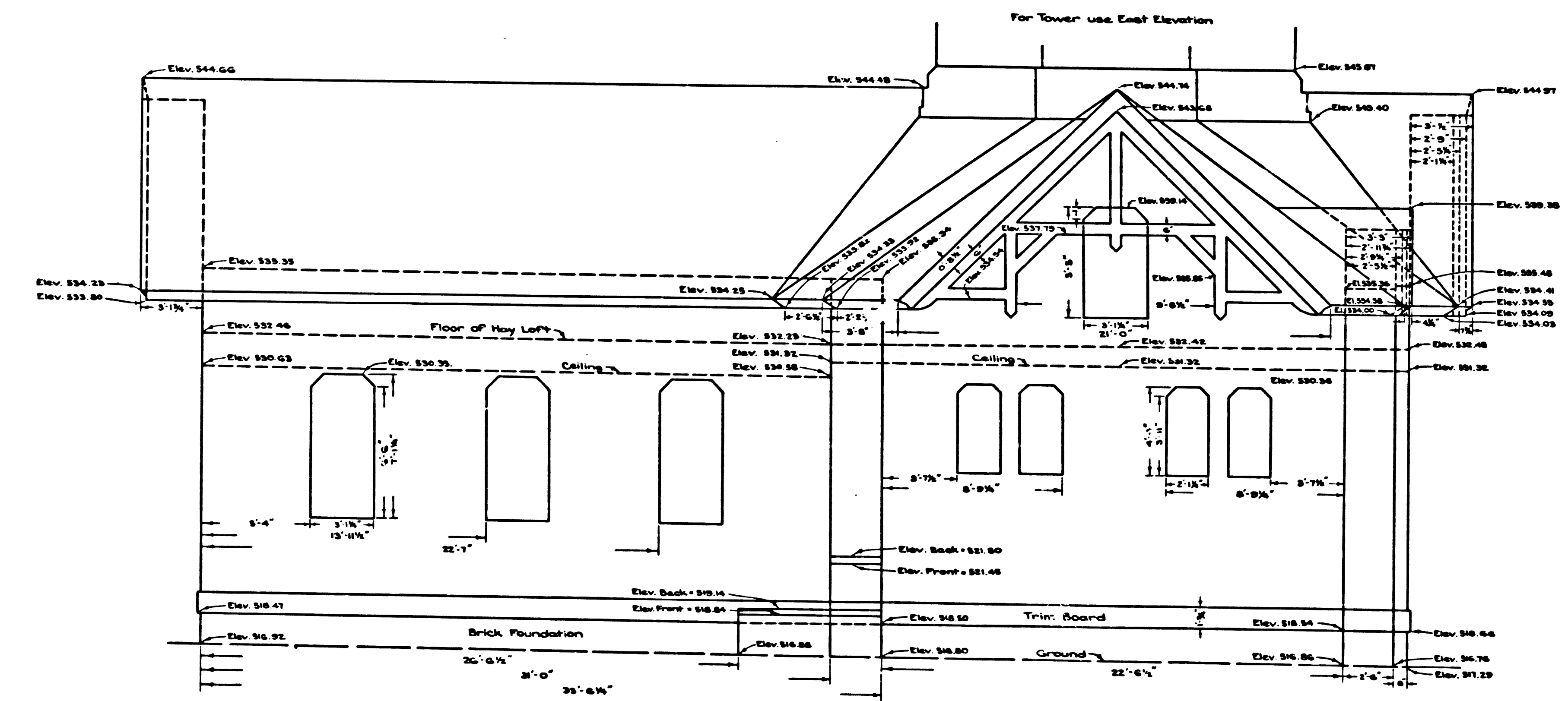
SOUTH ELEVATION
