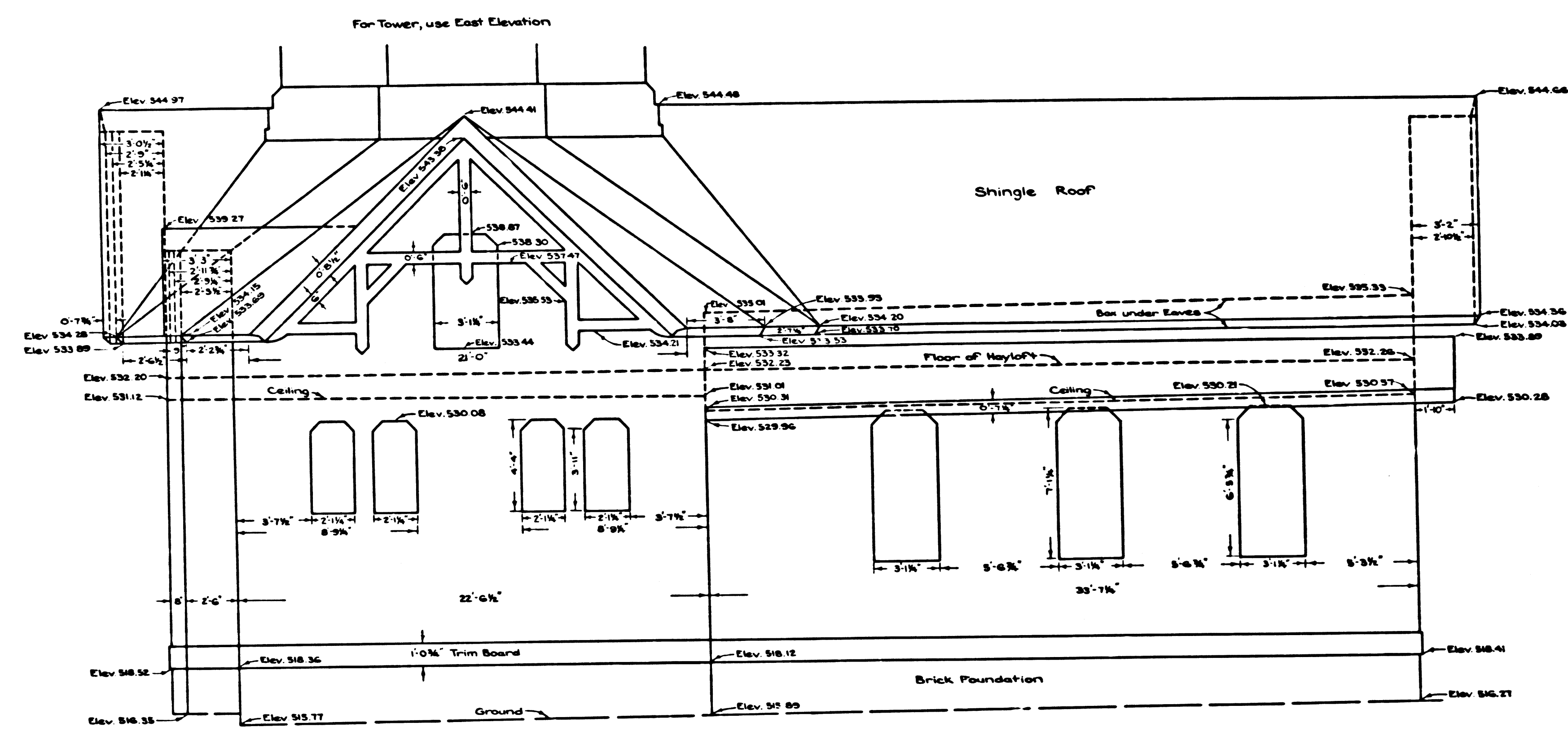
NORTH ELEVATION
