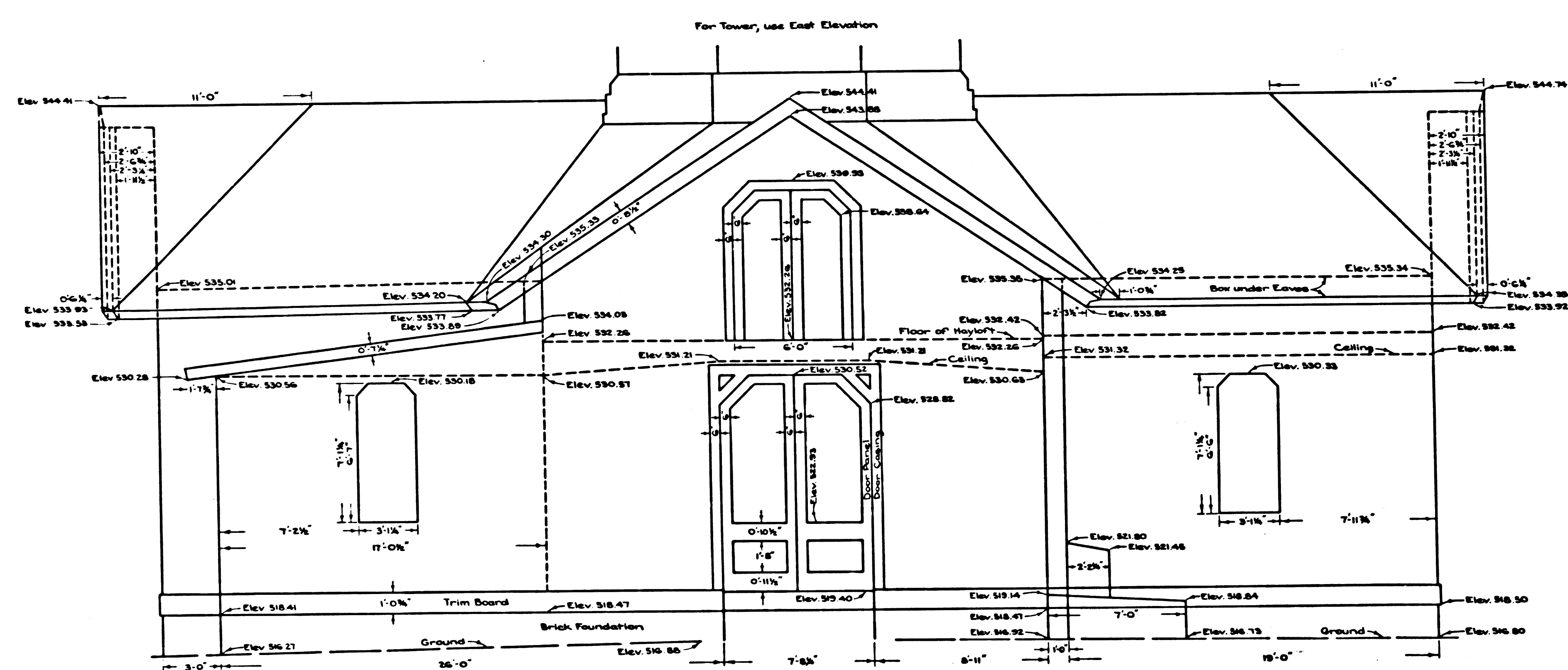
WEST ELEVATION
