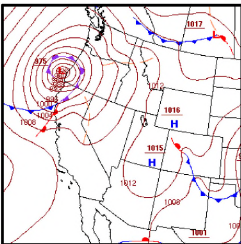
Current Surface Map 11/26/19 1600 PST
