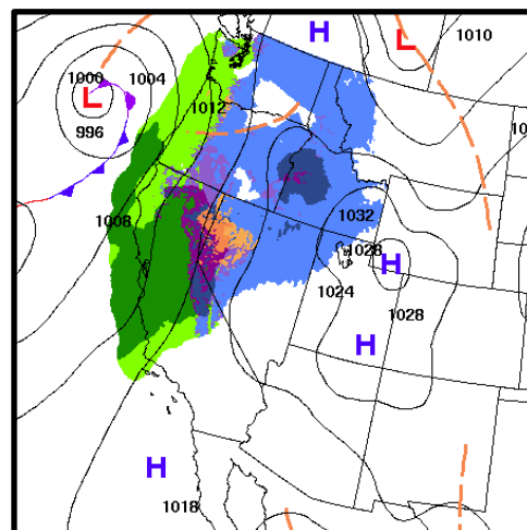
24 Hour Surface Forecast Map 12/1/19 1600 PST
