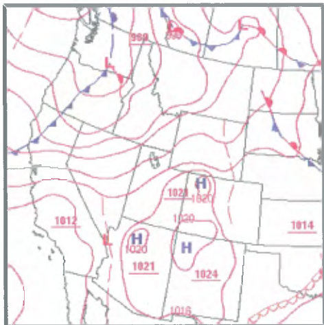
Current Surface Map 12/2/12 0400 PST
