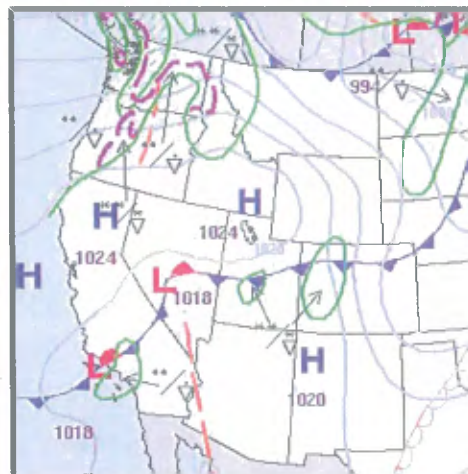
24 Hour Surface Forecast Map 12/3/12 0400 PST
