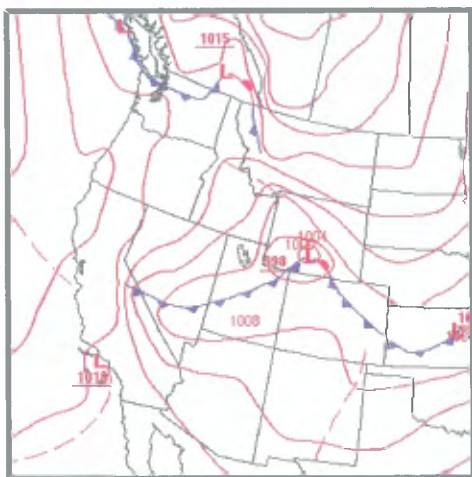
Current Surface Map 1/16/12 0400 PST
