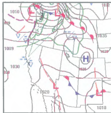
24 Hour Surface Forecast Map 1/17/12 0400 PST
