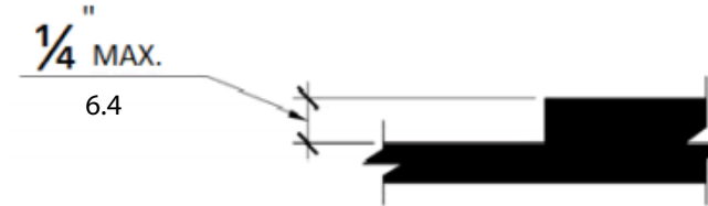
FIGURE 11B-303.2 VERTICAL CHANGE IN LEVEL
