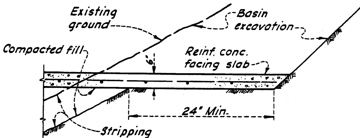
FACING SLAB DETAIL AT ABUTMENTS
