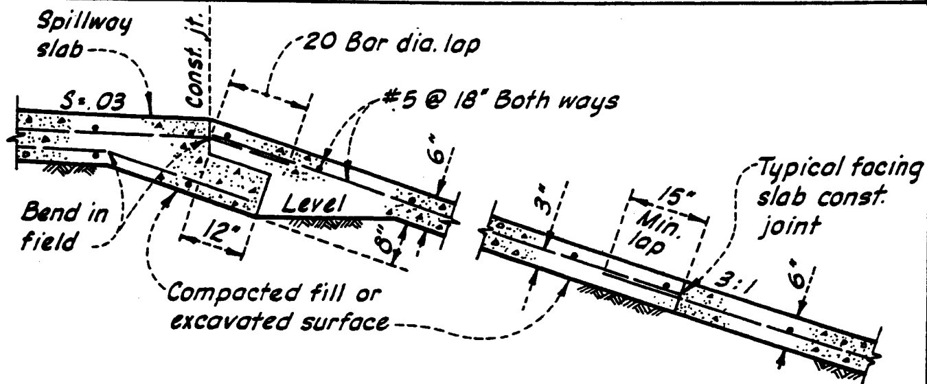
FACING SLAB DETAIL
