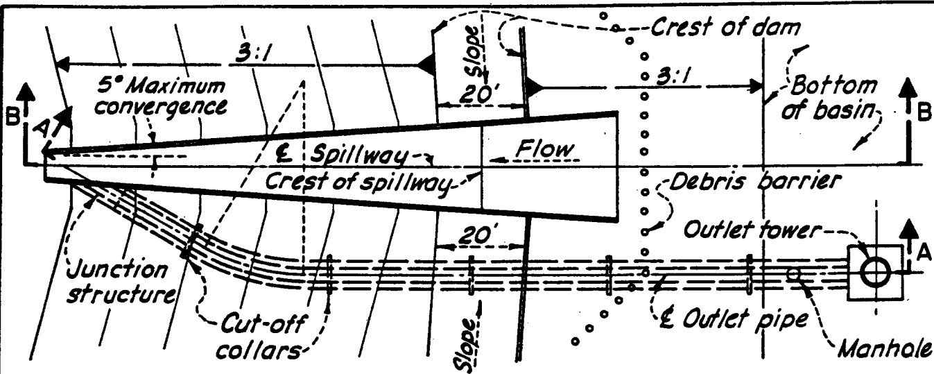
PLAN TYPICAL SPILLWAY AND OUTLET WORKS
