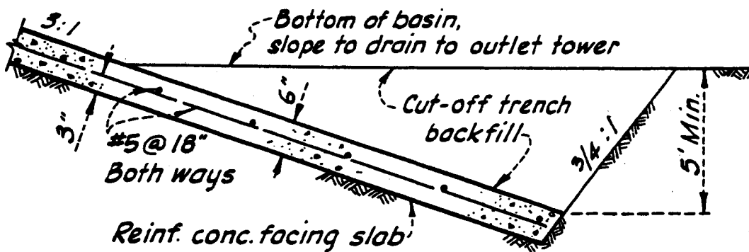
FACING SLAB CUT-OFF DETAIL
