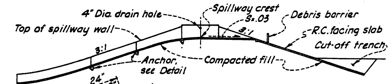
SECTION B-B
