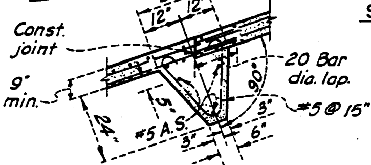
ANCHOR DETAIL
