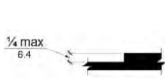
FIGURE 11B-303.2 VERTICAL CHANGE IN LEVEL
