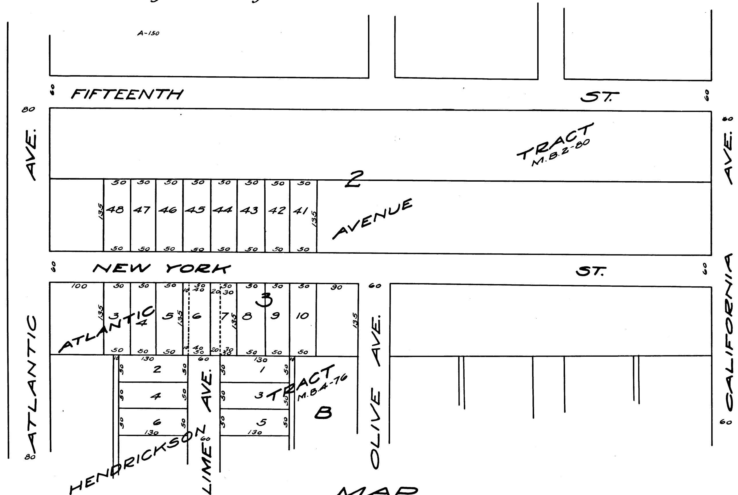
MAP Showing the opening & Extending of LIME AVE. in the City of Long Beach Scale 1"=100'
