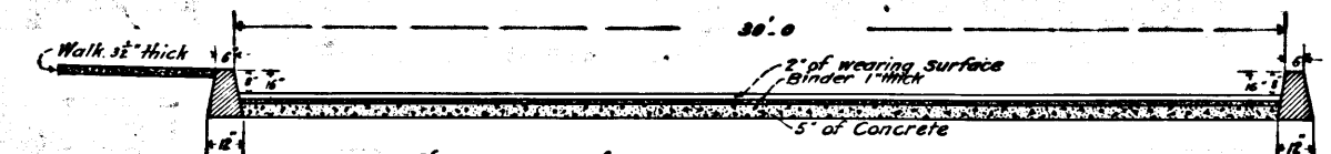
CROSS SECTION OF DRIVEWAY Scale: 1 in = 4 ft.
