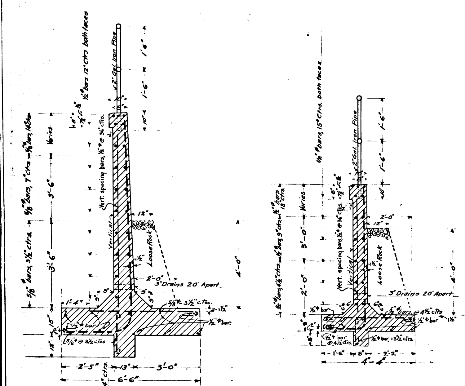
Section C-C Scale 1"=2' Section D-D Scale 1"=2'
