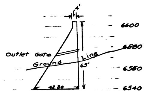
CROSS SECTION ALONG BB' Scale :- 1" = 50 Feet.
