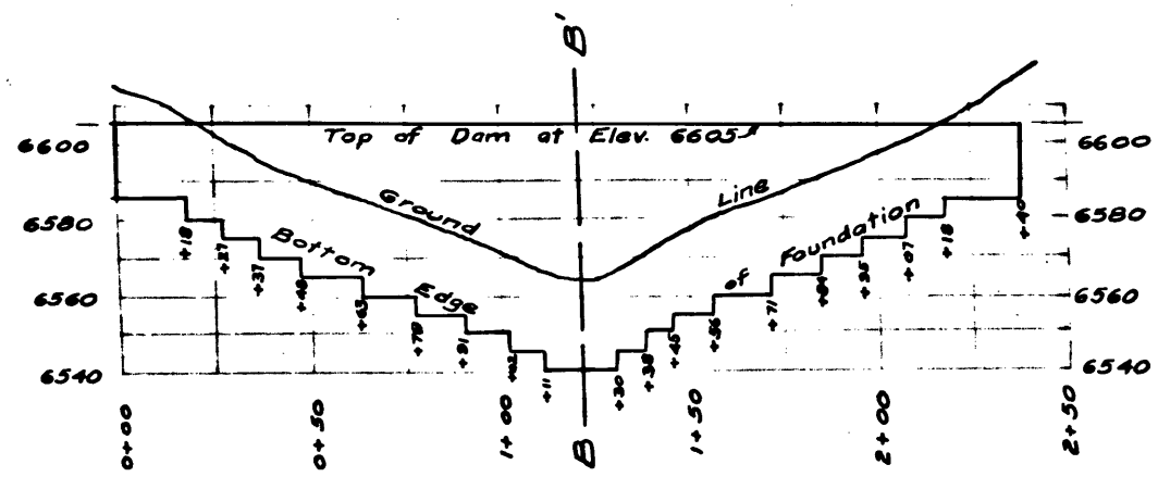
PROFILE ALONG LINE AA' Scale :- 1" = 50 Feet
