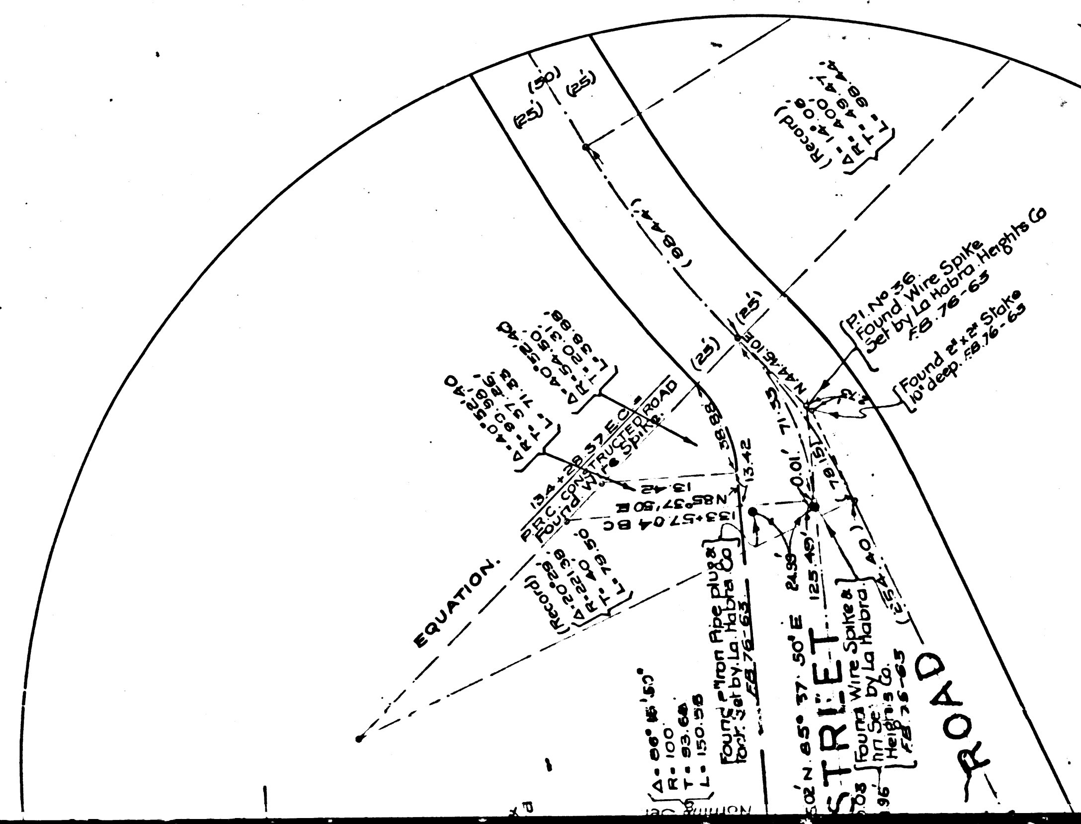
DETAIL OF INTERSECTION OF PROPOSED SIXTH STREET WITH WEST ROAD SCALE 1 INCH = 50'
