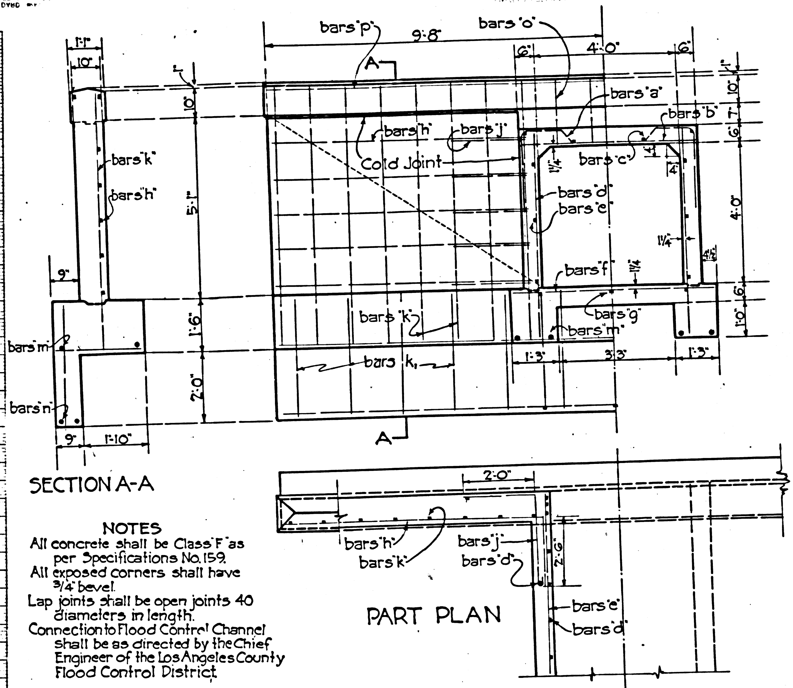
4x4' CONCRETE BOX- JUNE LANE & FERN LANE SCALE 1/2" = 1'-0"
