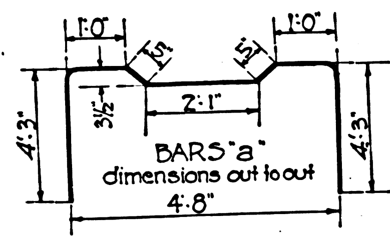
4x4' CONCRETE BOX- JUNE LANE & FERN LANE SCALE 1/2" = 1'-0"
