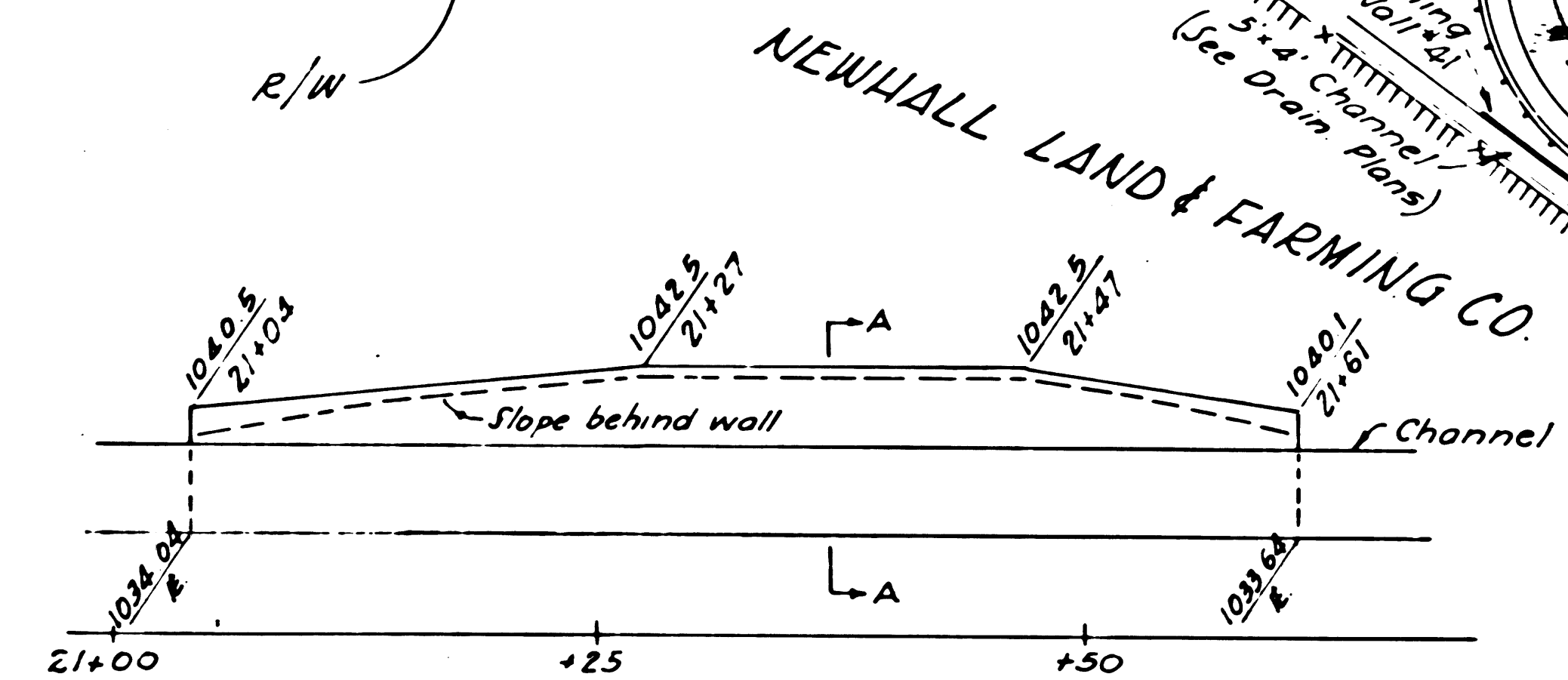
RETAINING WALL N° 41 Scale 1" = 10' TYPE I CANTILEVER RET. WALL
