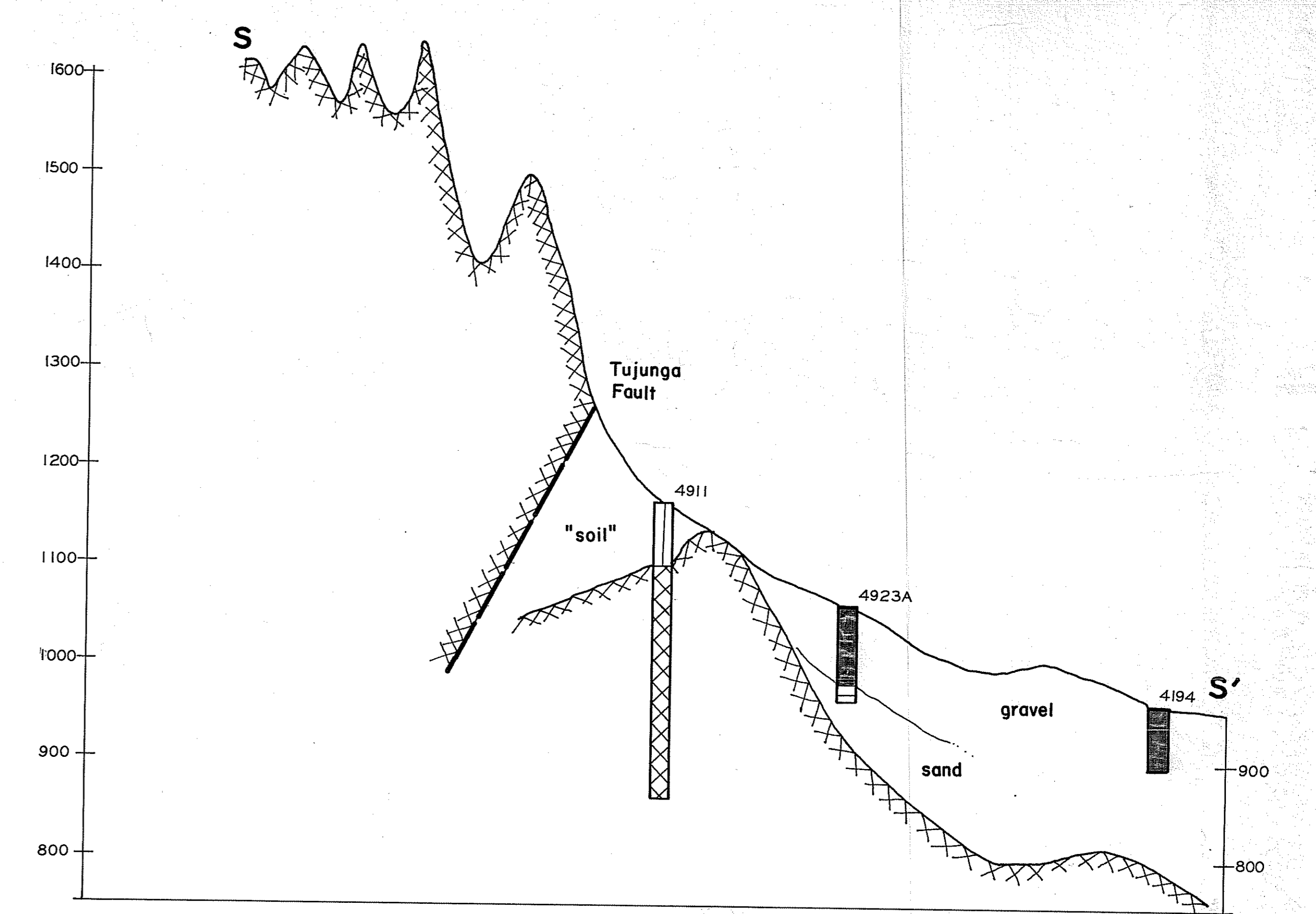
SOIL PROFILES P-P', Q-Q', S-S', R-R' AND T-T' See Plate 4 for Locations
