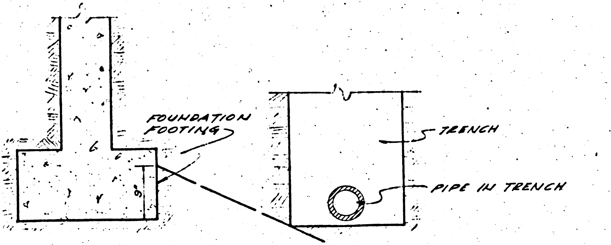
DETAIL OF PIPE TRENCH NEAR FOUNDATION NOT DRAWN TO SCALE
