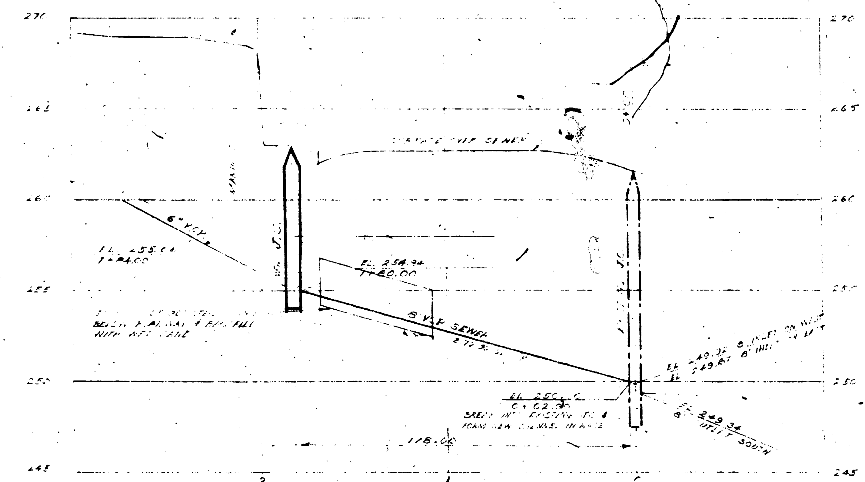
SEWER PROFILE SCALE HORIZONTAL 1" = 40' SCALE VERTICAL 1" = 4'
