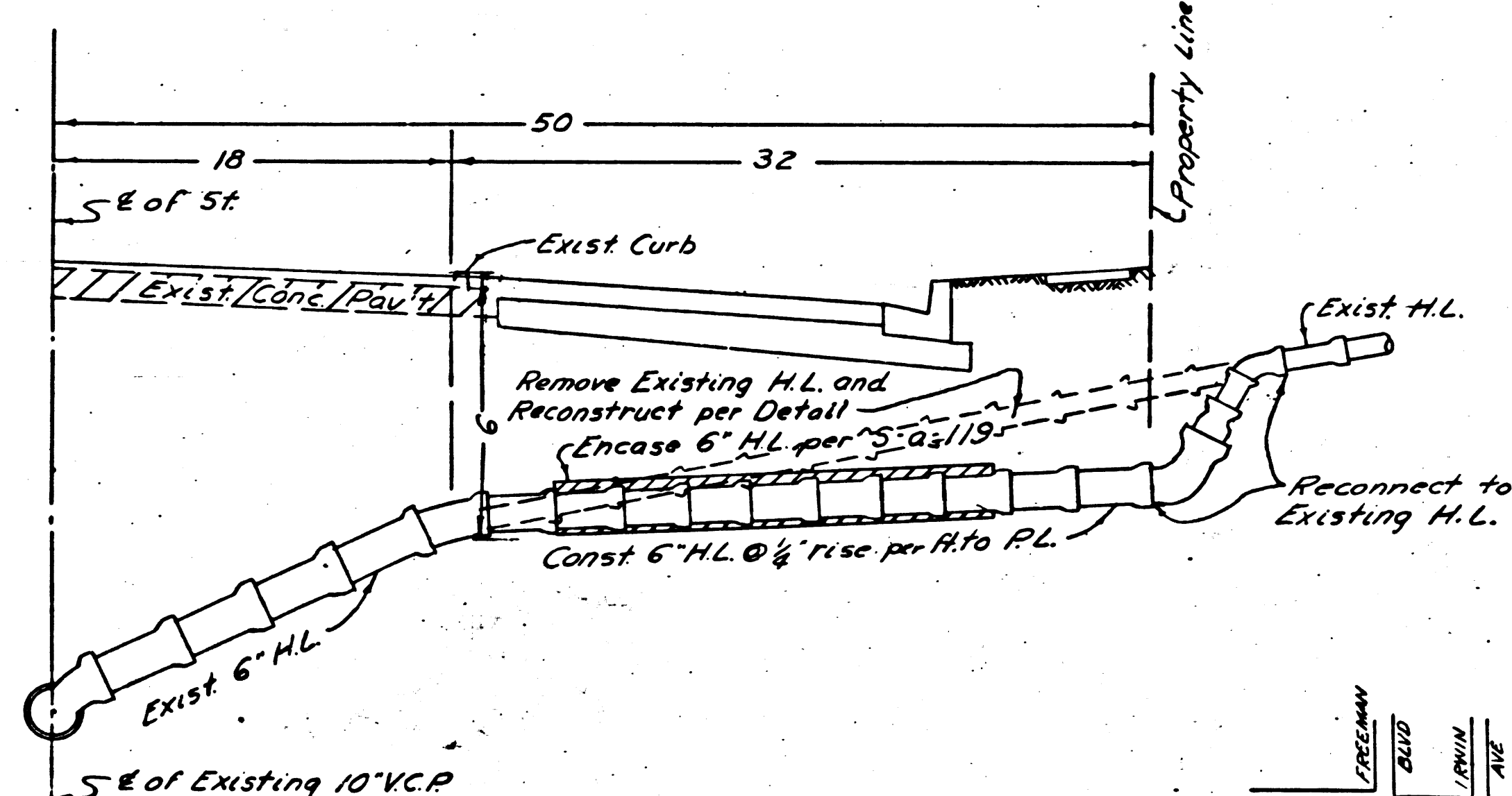
TYPICAL SECTION FOR RECONSTRUCTION OF EXISTING HOUSE LATERALS
