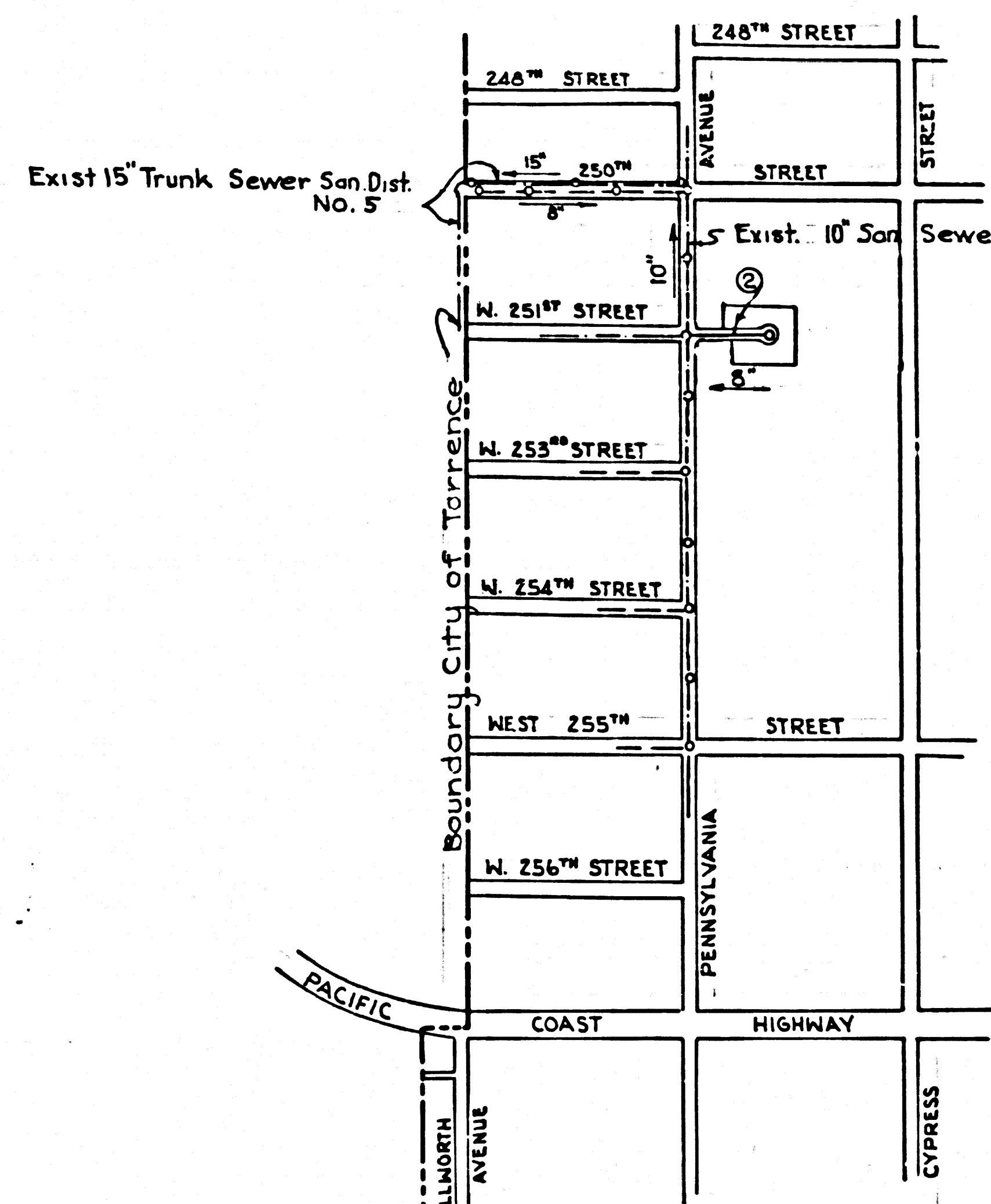
INDEX MAP TRACT NO. 25900 P.C. 5721 SCALE: 1"=60'
