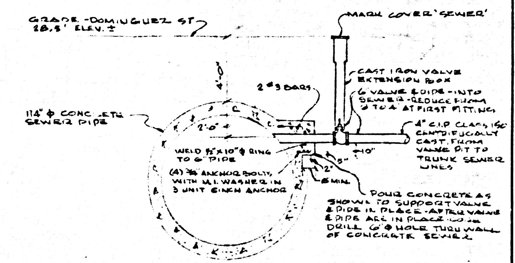
DETAIL - CONNECTION TO 114" ROUND SEWER NOT TO SCALE
