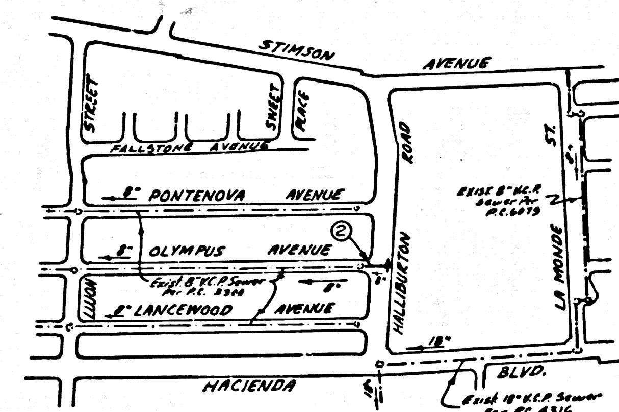
INDEX MAP SCALE: 1" = 600' P.C. 6997 OLYMPUS AVENUE
