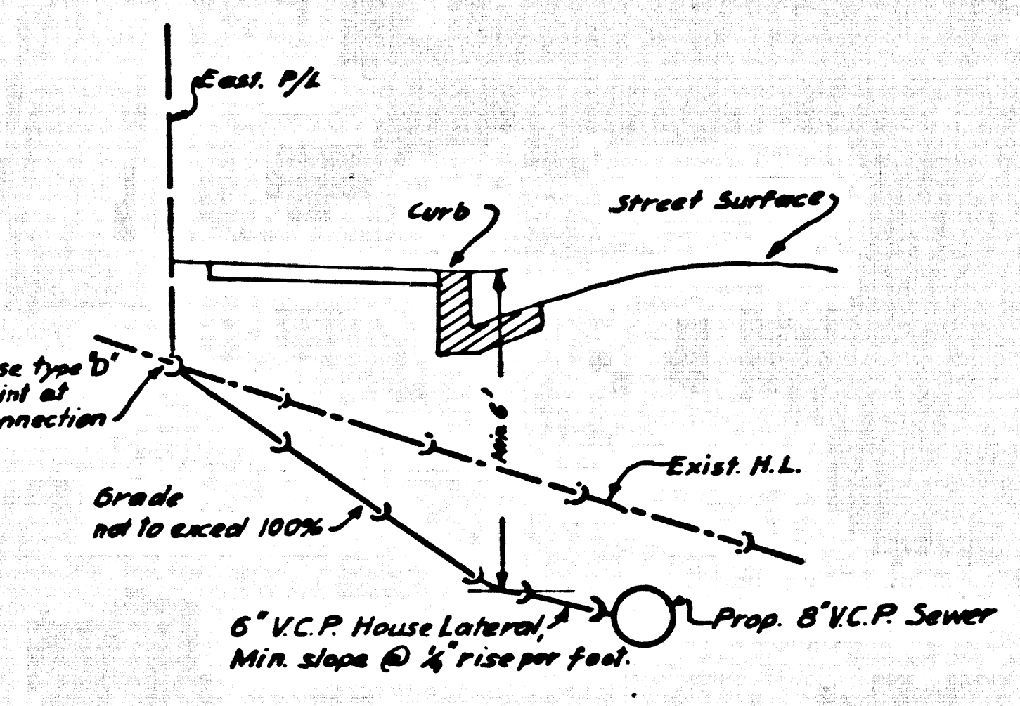
DETAIL HOUSE LATERAL RECONSTRUCTION NO SCALE
