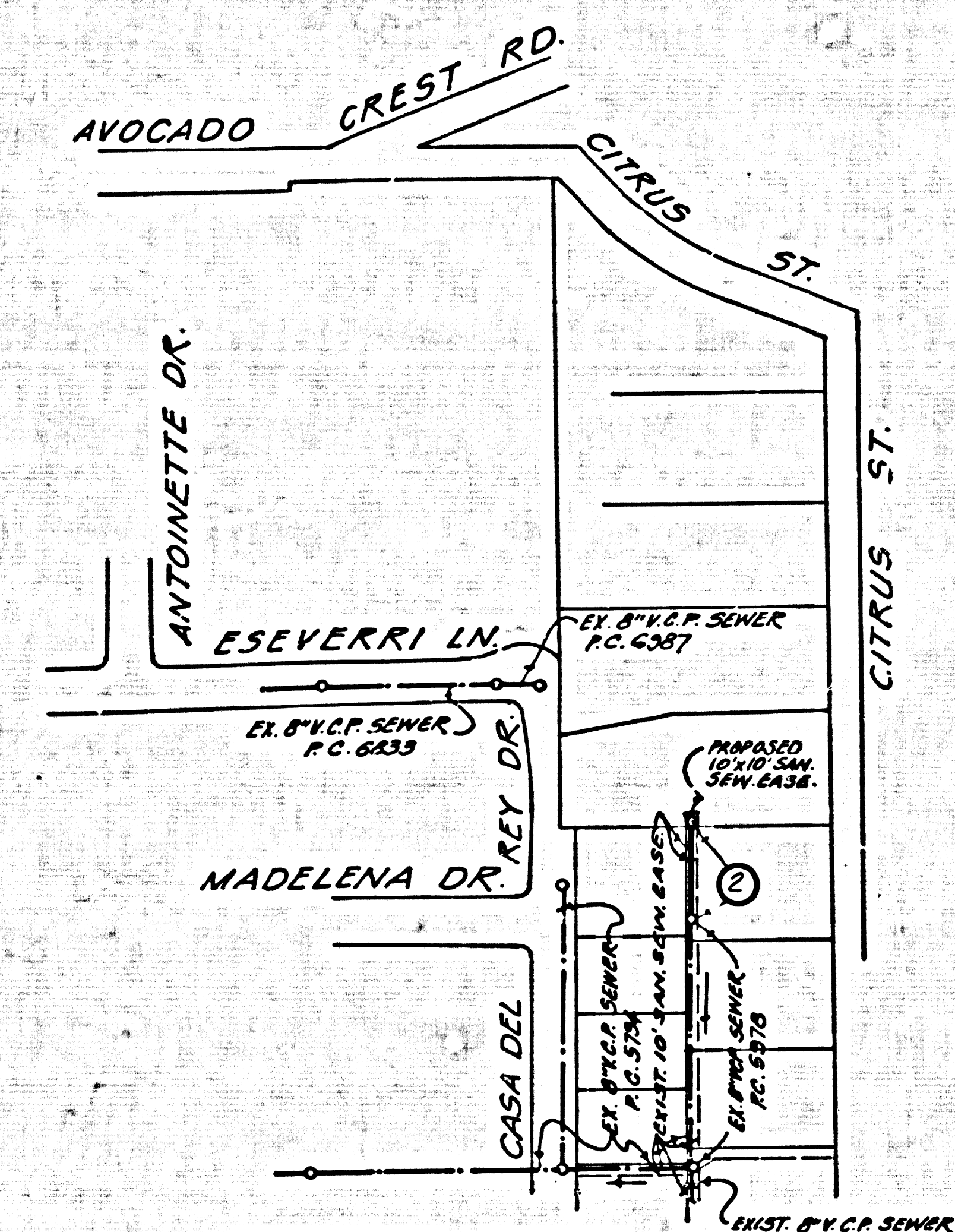
INDEX MAP SCALE: 1"=200' P. C. 9204
