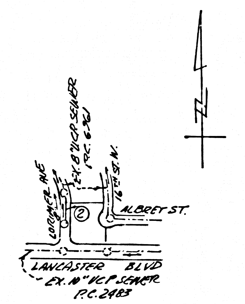
INDEX MAP SCALE 1"=600' P.C. 9392
