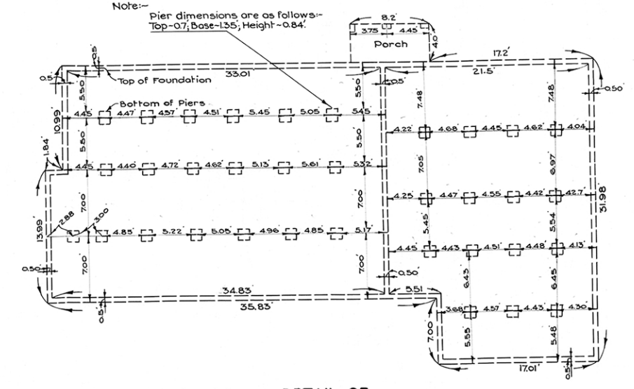
DETAIL OF PROPOSED FOUNDATION Scale: 1 inch = 8 feet
