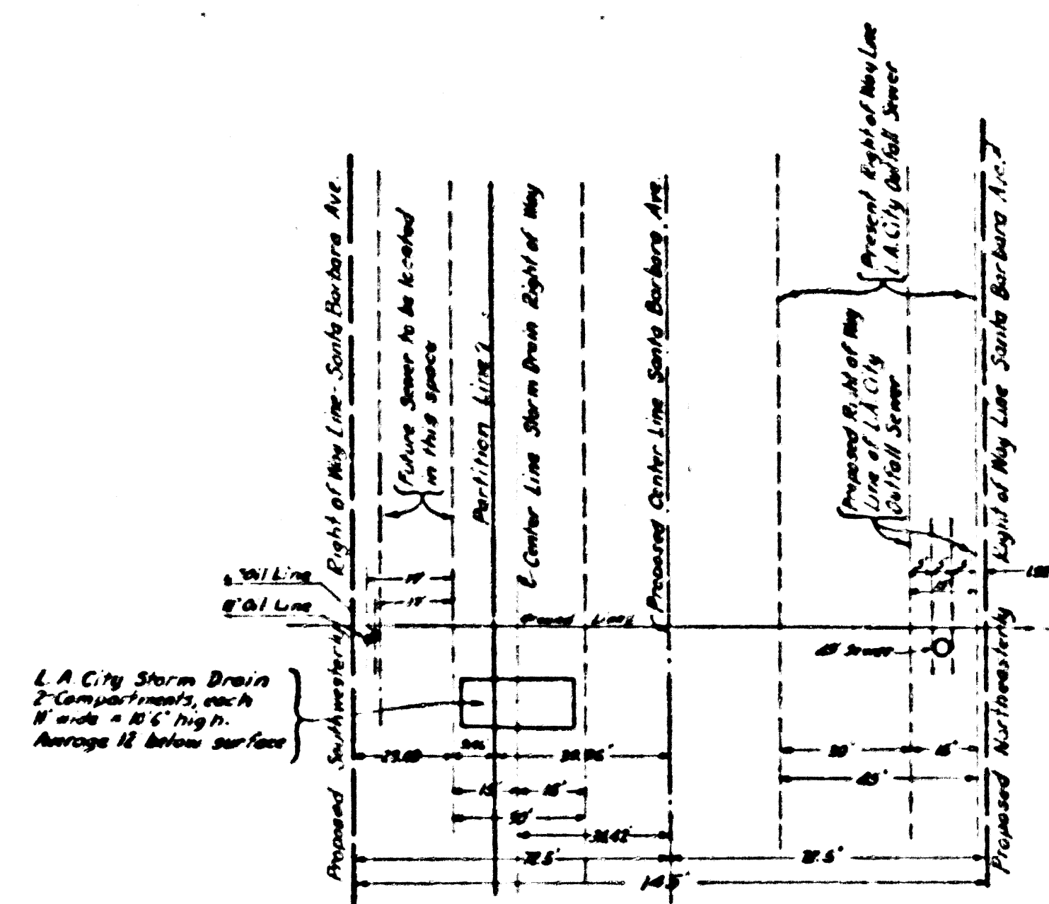
SKETCH SHOWING CROSS SECTION OF PROPOSED 145 FT SECTION OF SANTA BARBARA AVE. SCALE - 1 INCH = 30 FT.
