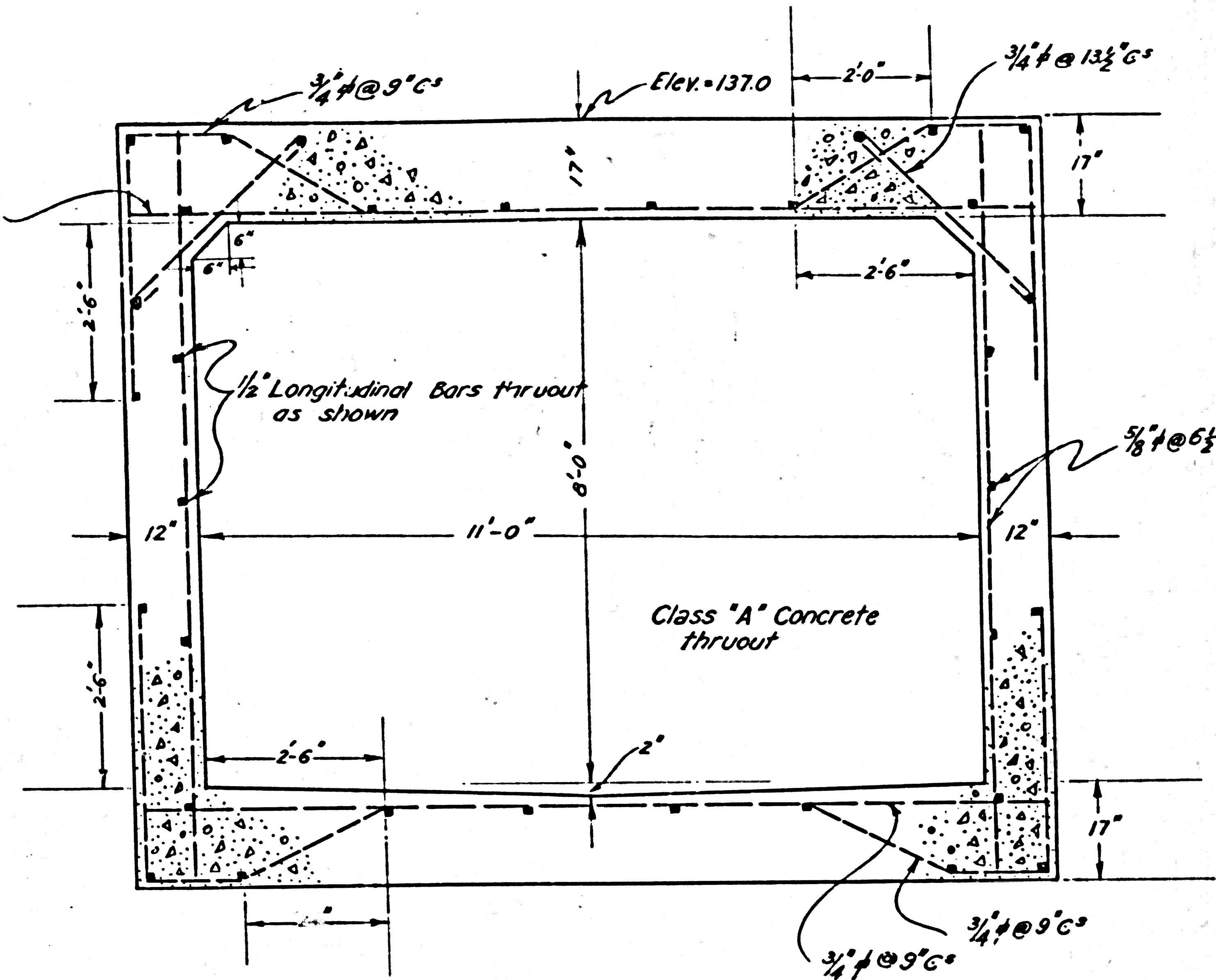
SECTION A-A Scale 1/2" = 1' 8'-0" x 11'-0" CONDUIT Under Pacific Electric Ry. Right of Way at WILSHIRE & EULALIA BLVDS. Length = 40'-0"
