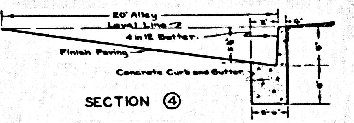
DETAIL OF ASPHALTIC CONCRETE PAVING EXCEPT AT AUTO PARKS
