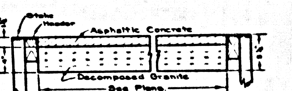
DETAIL OF ASPHALTIC CONCRETE PAVING EXCEPT AT AUTO PARKS
