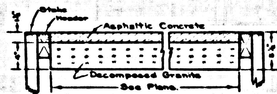
TYPICAL SECTIONS PER MECHANICAL DEPARTMENT PLANS
