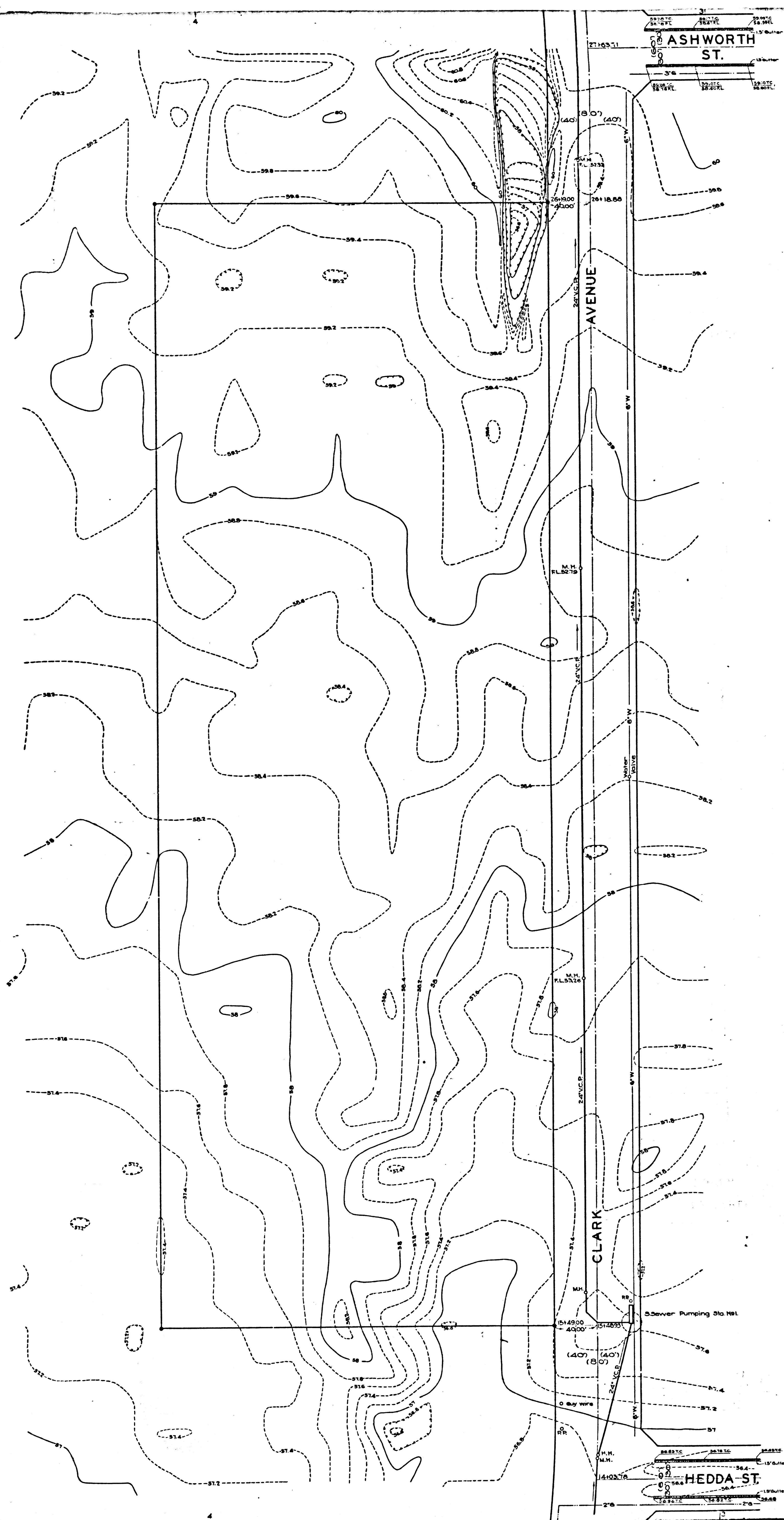
MARGINAL MAP SHOWING TOPOGRAPHY SCALE: 1 INCH = 40 FT. DATUM - MEAN SEA LEVEL ELEVATIONS SHOWN HEREON ARE BASED ON THE 1924 ADJUSTMENT OF U.S.C. & G.S. B.M. 5198 1922 (U.S. 2566) & 1168-1932 (U.S. 2926) & U.S. G.S. B.M. 75-1923 SIXBY (U.S. 2186)
