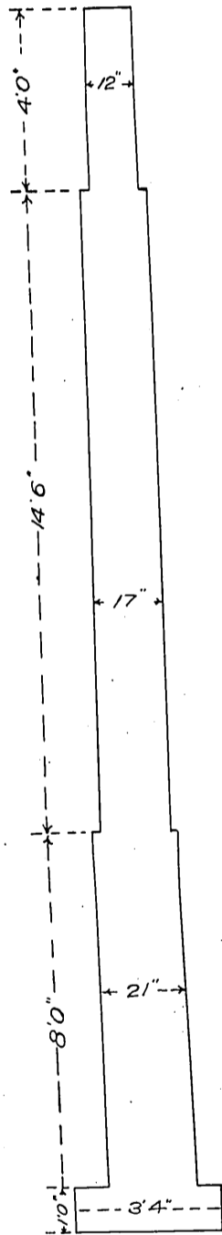
PARTY WALL Scale 1/4" to 1'
