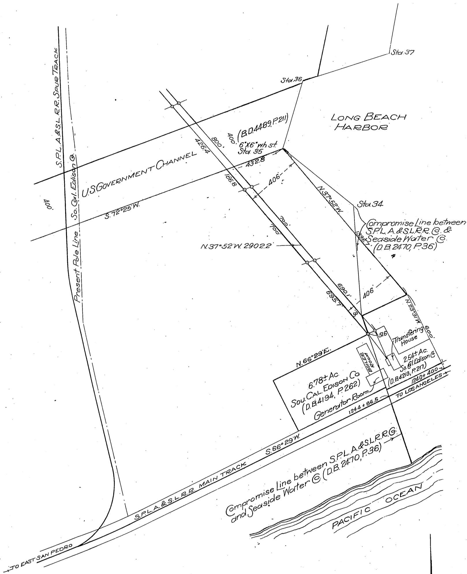
"EXHIBIT A" S.P.L.A. & S.L.R.R. LOS ANGELES DIVISION MAP OF LOCATION OF TRANSMISSION LINES SOUTHERN CALIFORNIA EDISON CO. OSTEND STATION LONG BEACH, CAL. SCALE 1 IN. = 400 FT.
