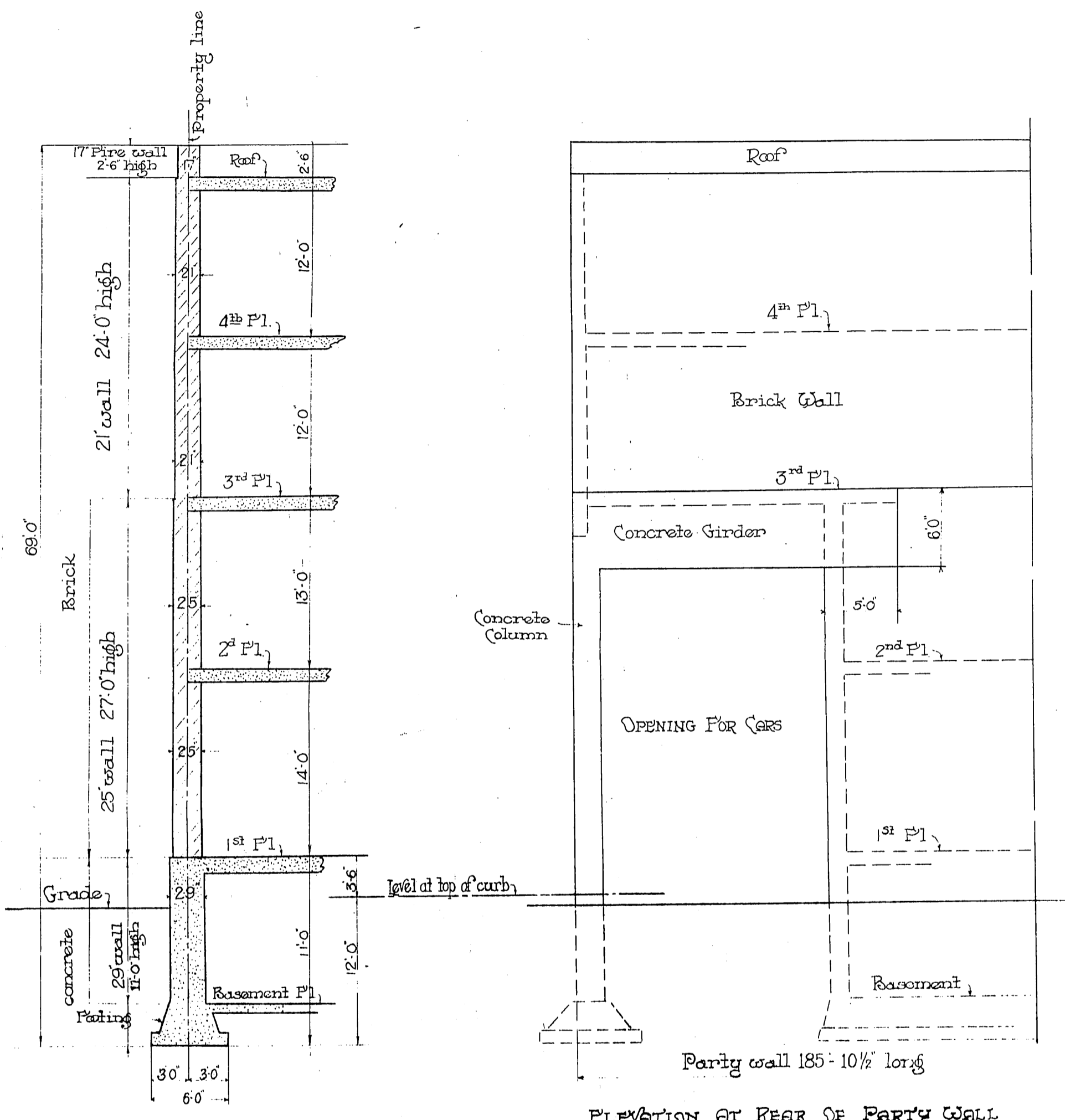
GENERAL SECTION PARTY WALL Scale 1/8" = 1'-0"
